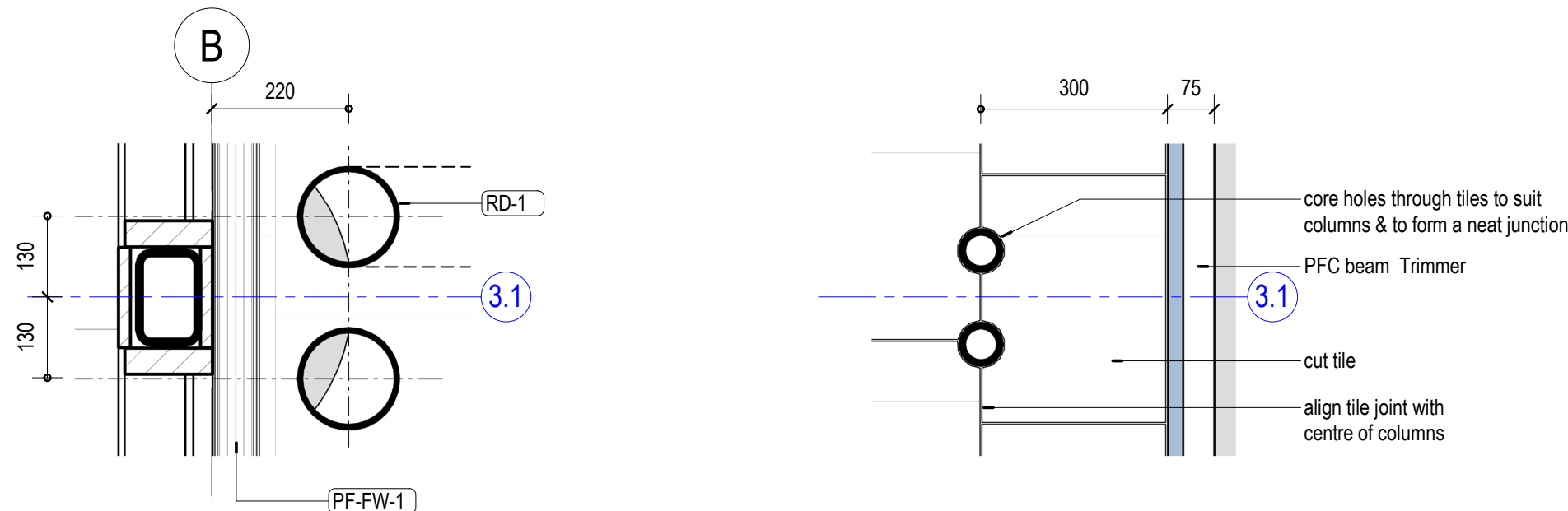
3 RD-1 Downpipe - Floor Detail 1 : 10 4 Twin Columns - Floor Detail 1 : 10
