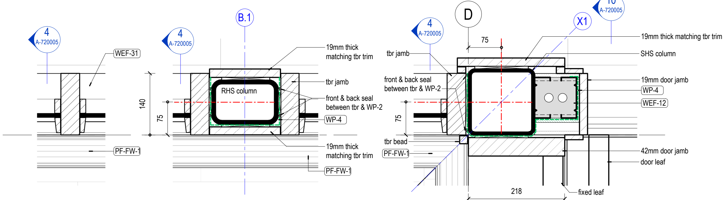
8 WEF23 Mullion 1 : 5 Courtyard 9 WEF23 Mullion @ Column 1 : 5 Courtyard 10 WEF23 Mullion @ Door 1 : 5 Courtyard
