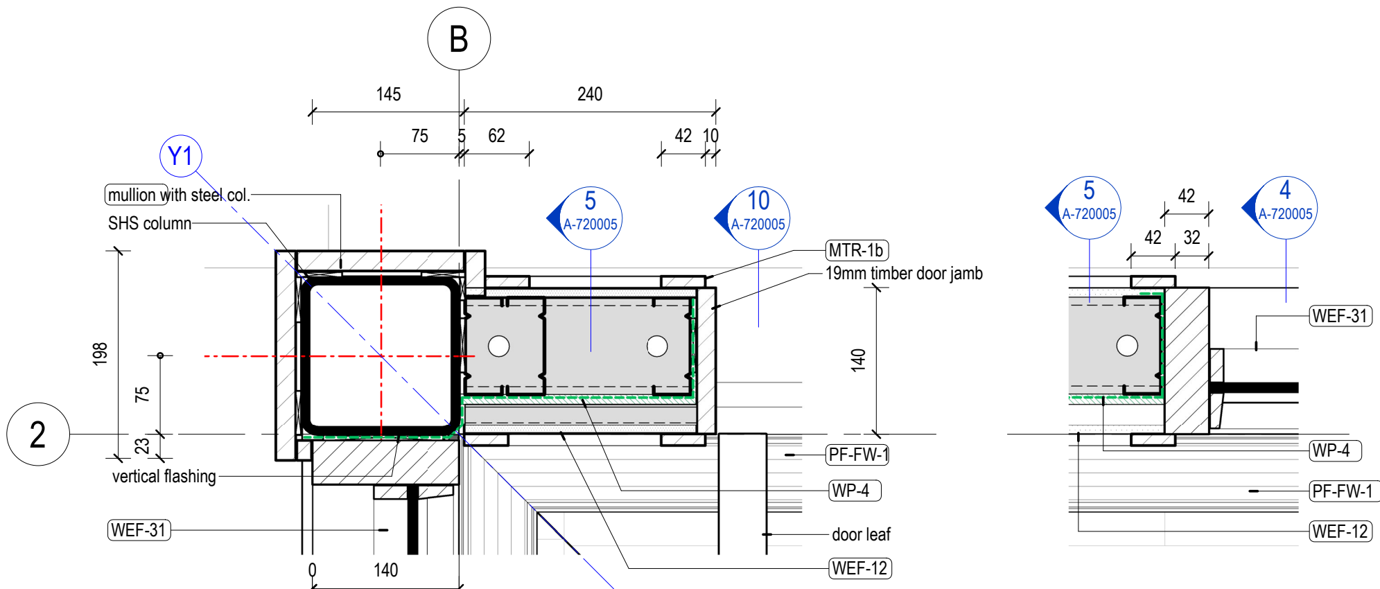
6 WEF-23 Corner Mullion 1 : 5 Courtyard 7 WEF-12 / WEF23 Junction 1 : 5 Courtyard
