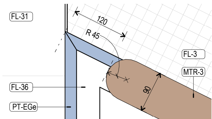
5 Courtyard - Bridge Hob 1 : 5
