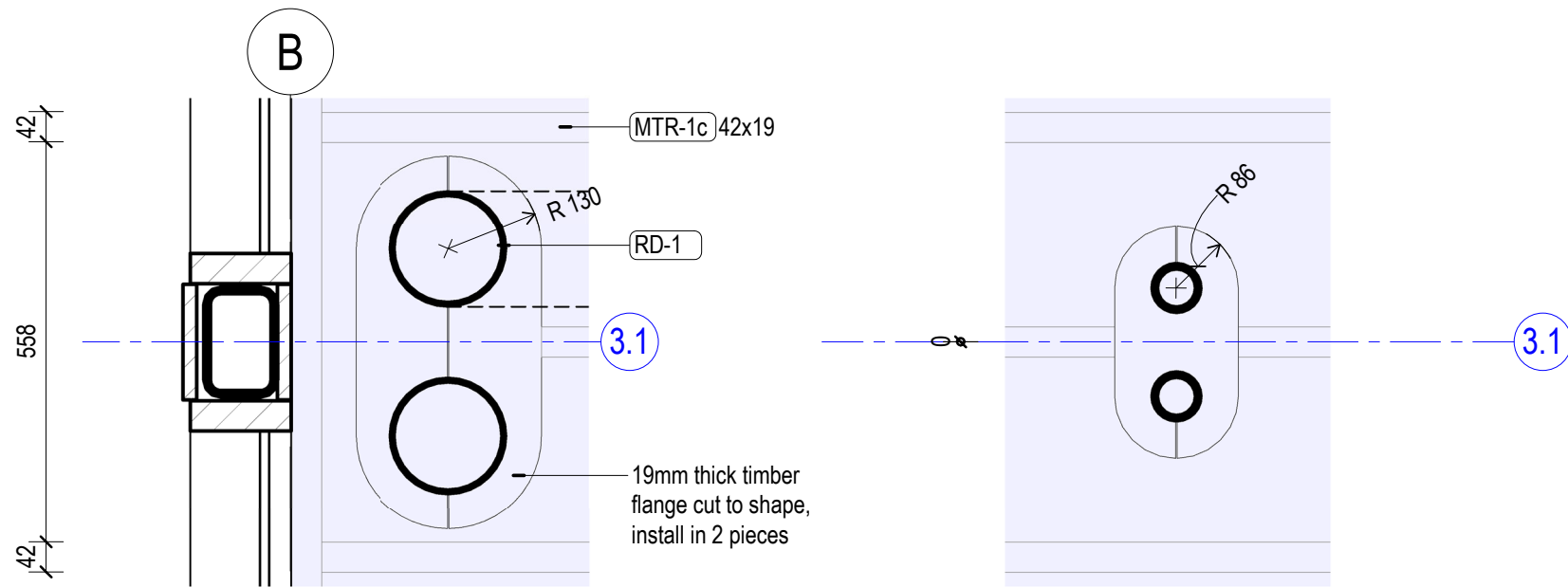
1 RD-1 Downpipe Ceiling Detail 1 : 10 2 Twin Columns - Ceiling Detail 1 : 10
